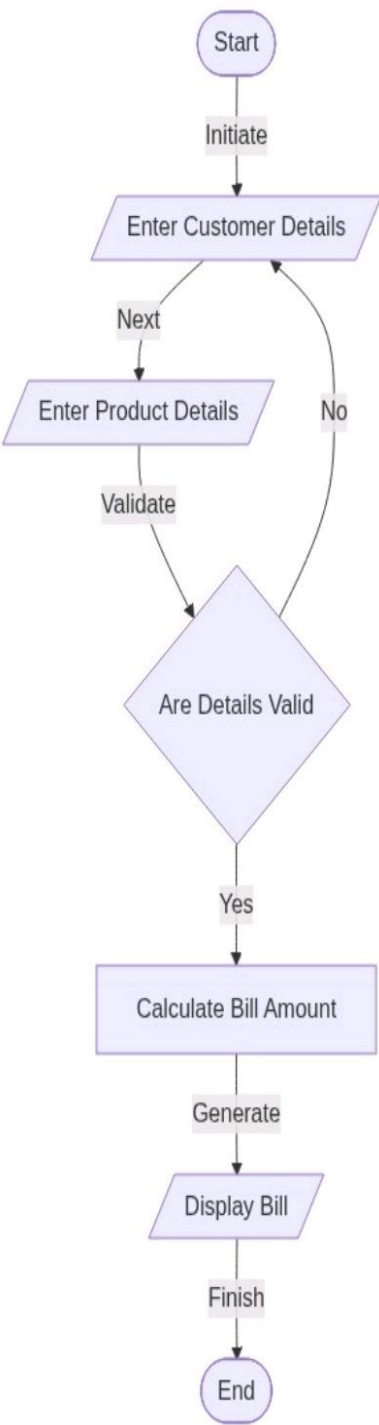
Customer Billing Flowchart
